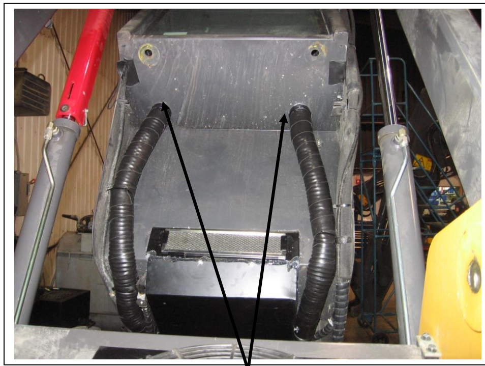
Hole saw and install louvers. Insulate 2 flex hoses and connect as shown.
